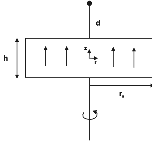
Fig.E2: Sketch of a homogeneously magnetized flat cylinder. The field shall be computed at a point with distance d from its upper face.
