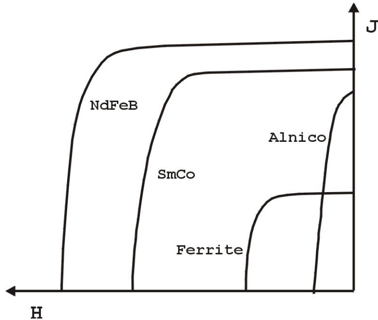
Fig.2: J(H) -curves for the most common permanent magnetic materials
